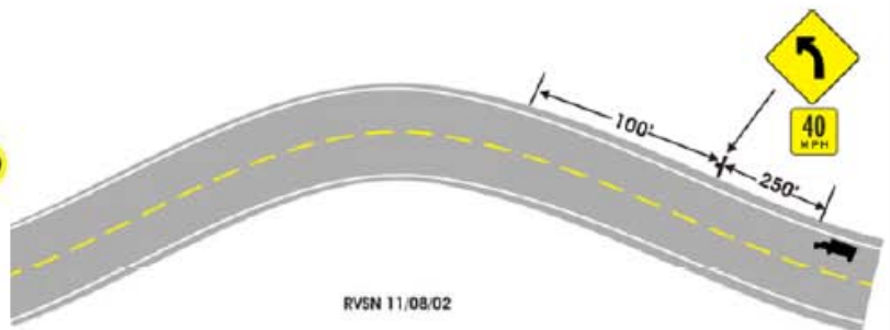
Advanced curve warning with speed limit
