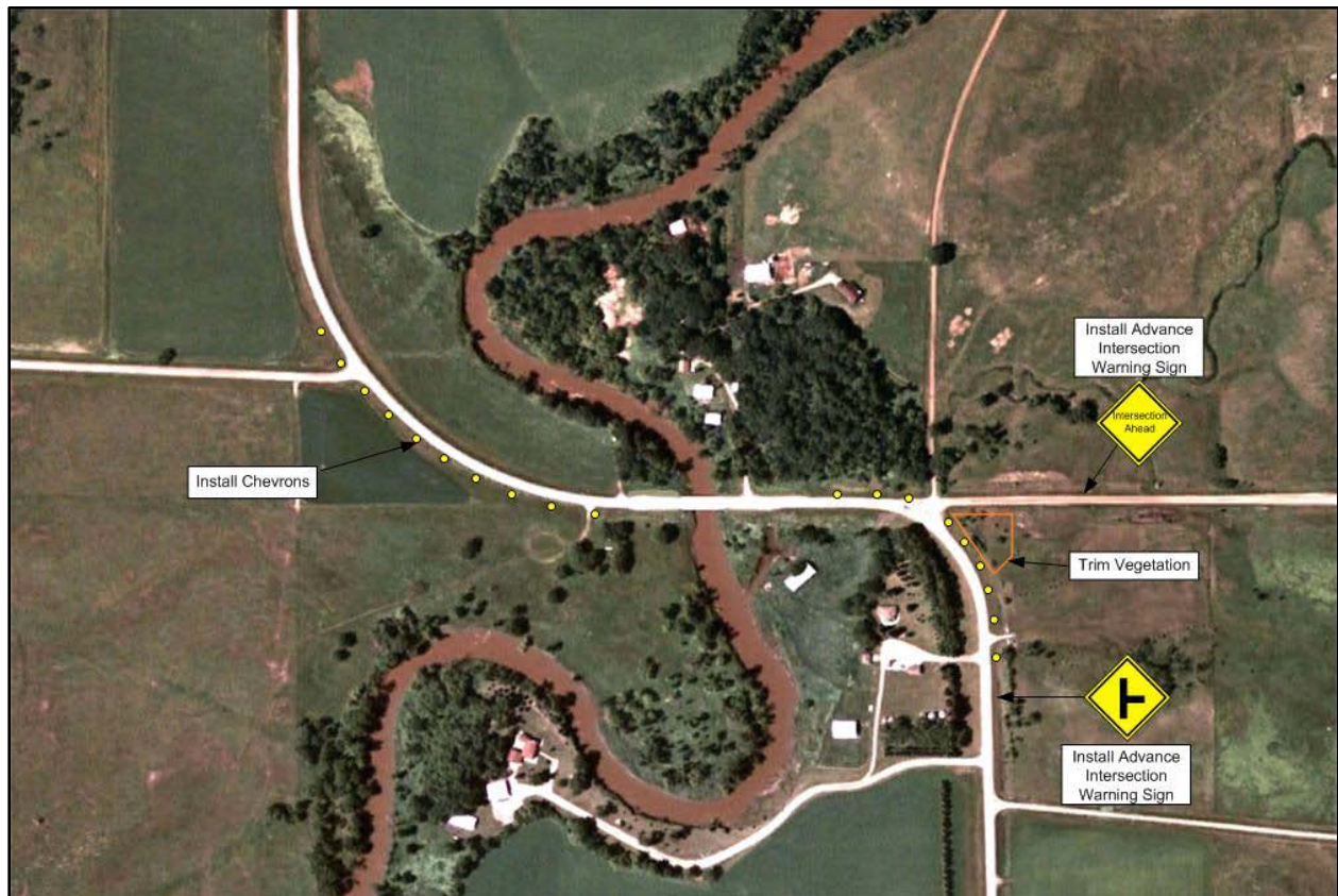
Figure 6.2 Short-term improvements for Skorpen Curve
